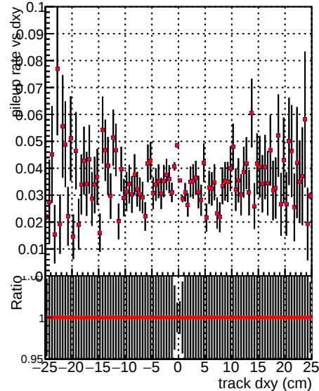
Global mkFit100dt RECO
