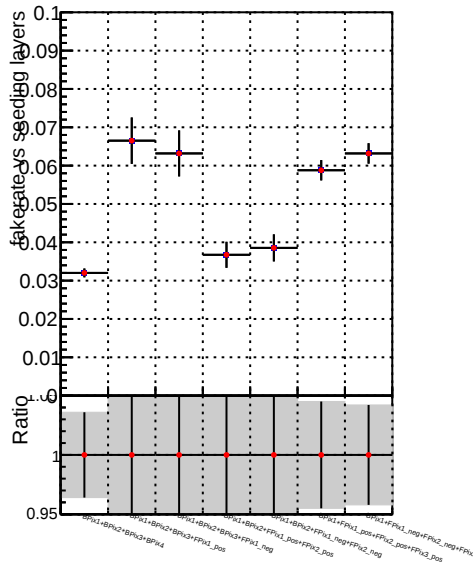
—•— DQM_V0001_R0000000001_Global_mkFit100o_RECO —•— DQM_V0001_R0000000001_Global_mkFit100dt_RECO
