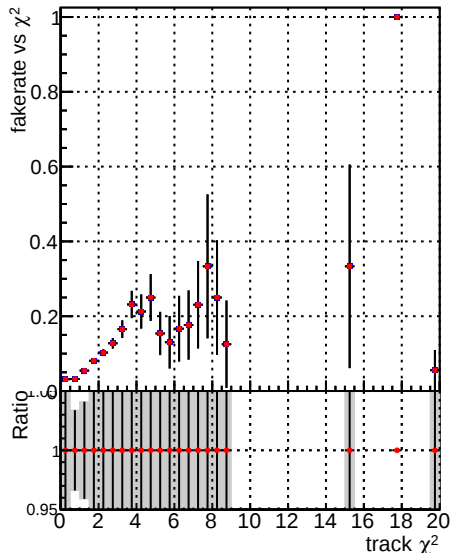
—•— DQM_V0001_R0000000001_Global_mkFit100o_RECO —•— DQM_V0001_R0000000001_Global_mkFit100dt_RECO
