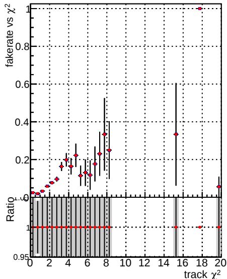
—●— DQM_V0001_R000000001_Global_mkFit100o_RECO —●— DQM_V0001_R000000001_Global_mkFit100dt_RECO
