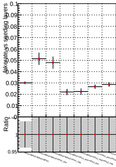
—●— DQM_V0001_R000000001_Global_mkFit100o_RECO —●— DQM_V0001_R000000001_Global_mkFit100dt_RECO
