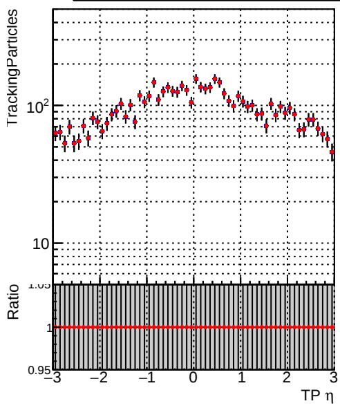
Legend: DQM_V0001_R000000001_Global_mkFit100o_RECO (blue dots), DQM_V0001_R000000001_Global_mkFit100dt_RECO (red dots)
