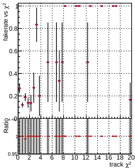
Fake rate vs. —•— DQM_V0001_R0000000001_Global_mkFit100o_RECO —•— DQM_V0001_R0000000001_Global_mkFit100dt_RECO
