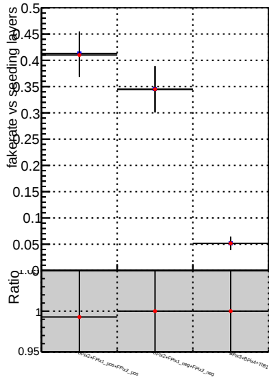
Fake rate vs. —•— DQM_V0001_R0000000001_Global_mkFit100o_RECO —•— DQM_V0001_R0000000001_Global_mkFit100dt_RECO
