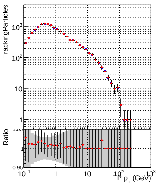
Legend: DQM_V0001_R000000001_Global_mkFit100o_RECO (blue dots), DQM_V0001_R000000001_Global_mkFit100dt_RECO (red dots)
