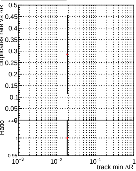
Legend: DQM_V0001_R000000001_Global_mkFit100o_RECO (black), DQM_V0001_R000000001_Global_mkFit100dt_RECO (red)
