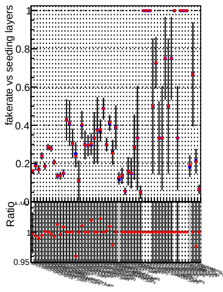
Fake rate vs. DQM V0001_R000000001 Global mkFit100o RECO DQM V0001_R000000001 Global mkFit100dt RECO
