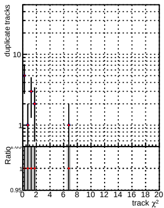
Legend: - Blue line: DQM_V0001_R0000000001_Global_mkFit100dt_RECO - Red line: DQM_V0001_R0000000001_Global_mkFit100dt_RECO - Grey histogram: verSet
