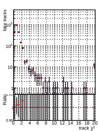
Legend: - Blue line: DQM_V0001_R0000000001_Global_mkFit100dt_RECO - Red line: DQM_V0001_R0000000001_Global_mkFit100dt_RECO - Grey histogram: verSet
