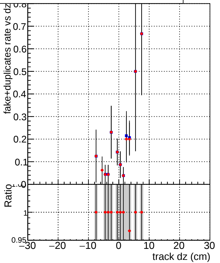
DQM_V0001_R000000001_Global_mkFit100o_RECO DQM_V0001_R000000001_Global_mkFit100dt_RECO
