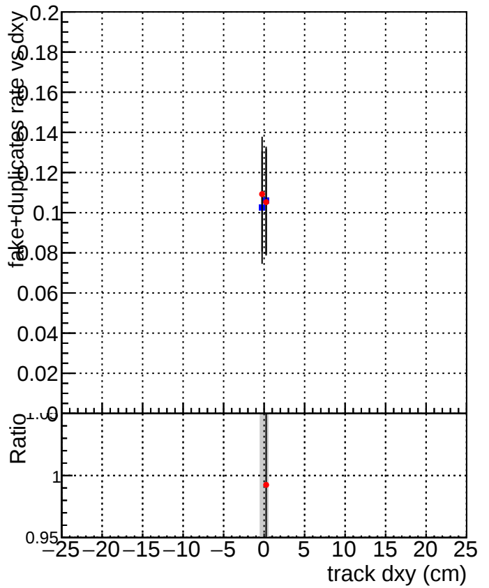
DQM_V0001_R000000001_Global_mkFit100o_RECO DQM_V0001_R000000001_Global_mkFit100dt_RECO
