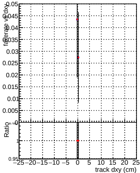
—●— DQM_V0001_R0000000001_Global_mkFit100o_RECO —●— DQM_V0001_R0000000001_Global_mkFit100dt_RECO
