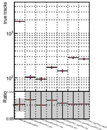
N of reco track vs. \chi^2 — Global_mkFit100o_RECO — Global_mkFit100dt_RECO
