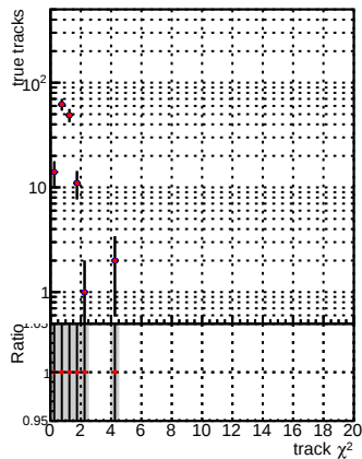
N of reco track vs. \chi^2 for DQM_V0001_R0000000001_Global_mkFit100o_RECO (blue) and DQM_V0001_R0000000001_Global_mkFit100dt_RECO (red).
