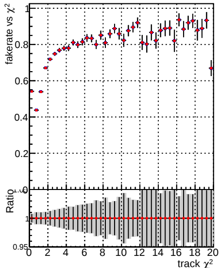
Fake rate vs. DQM_V0001_R0000000001 Global mkFit100o RECO
