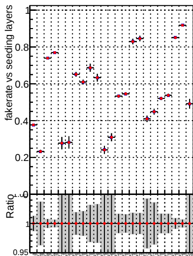
Fake rate vs. DQM_V0001_R0000000001 Global mkFit100o RECO
