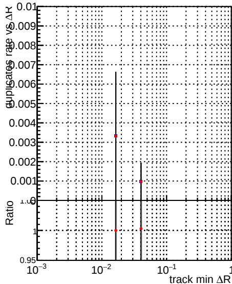
—●— DQM_V0001_R000000001_Global_mkFit100o_RECO —●— DQM_V0001_R000000001_Global_mkFit100dt_RECO
