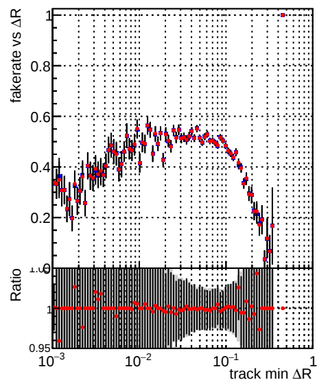
—●— DQM_V0001_R000000001_Global_mkFit100o_RECO —●— DQM_V0001_R000000001_Global_mkFit100dt_RECO
