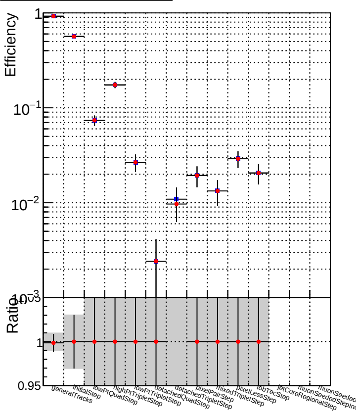
DQM_V0001_R000000001_Global_mkFit100o_RECO DQM_V0001_R000000001_Global_mkFit100dt_RECO
