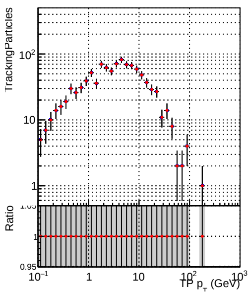
— DQM_V0001_R0000000001_Global_mkFit100o_RECO — DQM_V0001_R0000000001_Global_mkFit100dt_RECO
