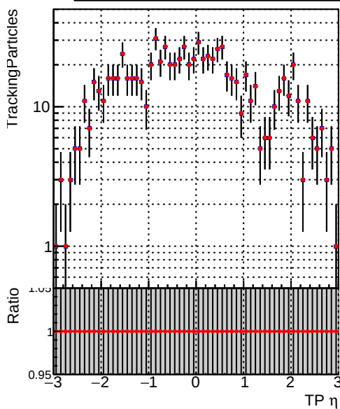
— DQM_V0001_R0000000001_Global_mkFit100o_RECO — DQM_V0001_R0000000001_Global_mkFit100dt_RECO
