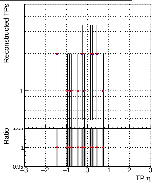
— DQM_V0001_R0000000001_Global_mkFit100o_RECO — DQM_V0001_R0000000001_Global_mkFit100dt_RECO
