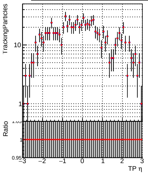
Legend: DQM_V0001_R000000001_Global_mkFit100o_RECO (blue line), DQM_V0001_R000000001_Global_mkFit100dt_RECO (red line)
