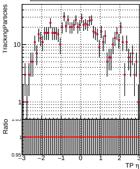
N of simulated tracks vs \eta Legend: DQM_V0001_R000000001_Global_mkFit100o_RECO (blue line), DQM_V0001_R000000001_Global_mkFit100dt_RECO (red line)
