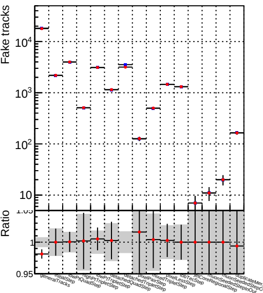
Number Label 1 DQM_V0001_R0000000001_Global_mkFit100dt_RECO
