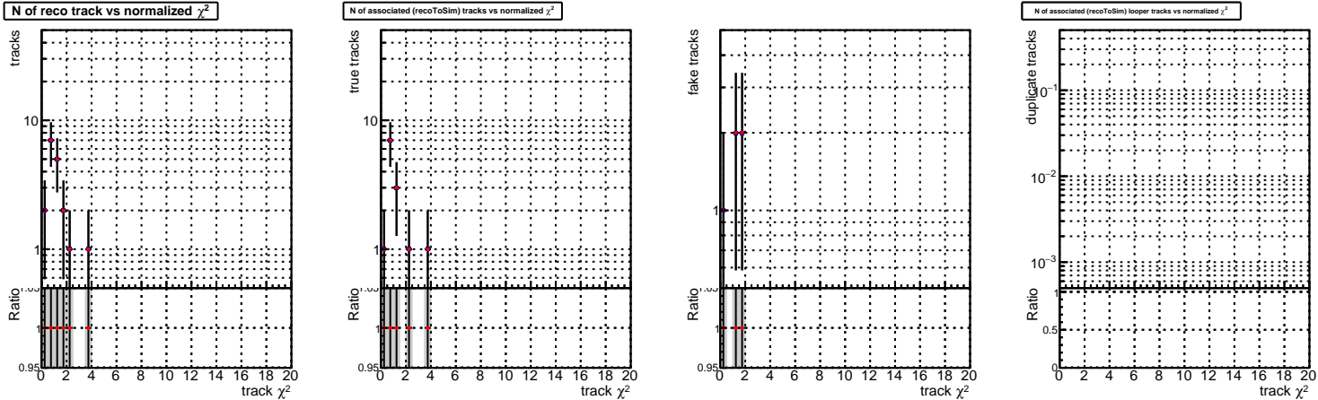
N of reco track vs. \chi^2 DQM_V0001_R0000000001_Global_mkFit100o_RECO DQM_V0001_R0000000001_Global_mkFit100dt_RECO
