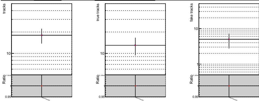
N of reco track vs. \chi^2 DQM_V0001_R0000000001_Global_mkFit100o_RECO DQM_V0001_R0000000001_Global_mkFit100dt_RECO
