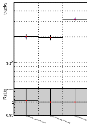
N of reco track vs. \chi^2 DQM_V0001_R0000000001_Global_mkFit100a_RECO DQM_V0001_R0000000001_Global_mkFit100dt_RECO
