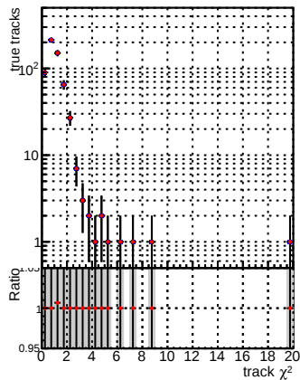
N of reco track vs. \chi^2 DQM_V0001_R0000000001_Global_mkFit100a_RECO DQM_V0001_R0000000001_Global_mkFit100dt_RECO
