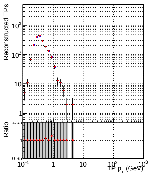
Legend: DQM_V0001_R0000000001_Global_mkFit100o_RECO (blue line with dots), DQM_V0001_R0000000001_Global_mkFit100dt_RECO (red line with dots)
