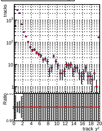
N of reco track vs. —●— DQM_V0001_R0000000001_Global_mkFit100o_RECO —●— DQM_V0001_R0000000001_Global_mkFit100dt_RECO
