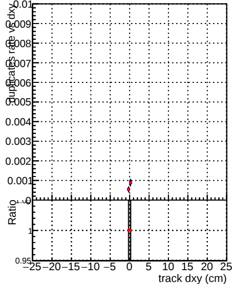
—•— DQM_V0001_R0000000001_Global_mkFit100o_RECO —•— DQM_V0001_R0000000001_Global_mkFit100dt_RECO
