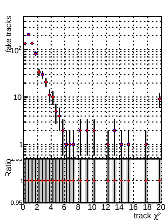
Legend: - Blue line: DQM_V0001_R000000001_Global_mkFit1000a_RECO - Red line: DQM_V0001_R000000001_Global_mkFit1000dt_RECO - Grey shaded region: verSet
