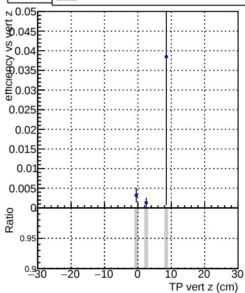
Efficiency vs. TP vert z (cm) DQM_V0001_R0000000001_Global_mkFit100_RECO
