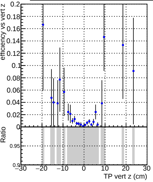
Efficiency vs TP vert r (cm) DQM_V0001_R000000001_Global_mkFit100_RECO
