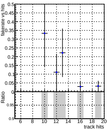
DQM_V0001_R000000001_Global_mkFit100_RECO
