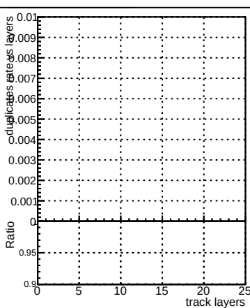
DQM_V0001_R000000001_Global_mkFit100_RECO
