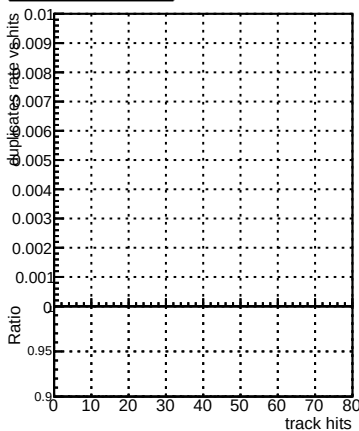
DQM_V0001_R000000001_Global_mkFit100_RECO
