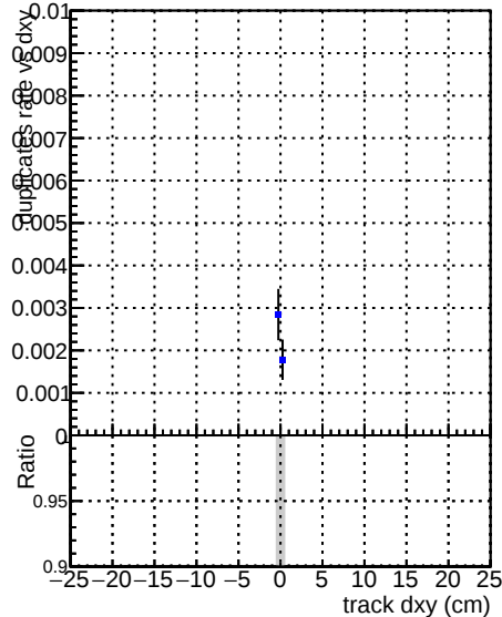
DQM_V0001_R000000001_Global_mkFit100_RECO
