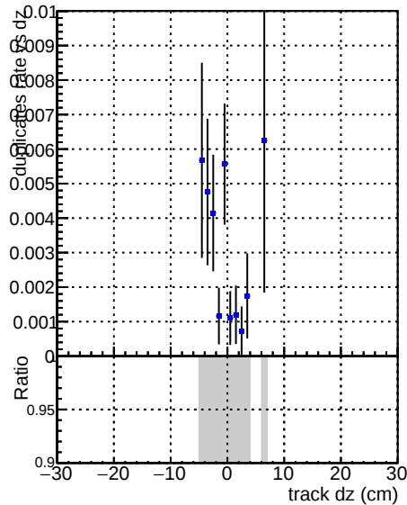
DQM_V0001_R000000001_Global_mkFit100_RECO
