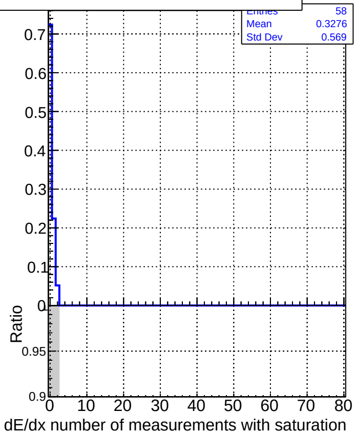
DQM_V0001_R000000001_Global_mkFiti100_RECO
