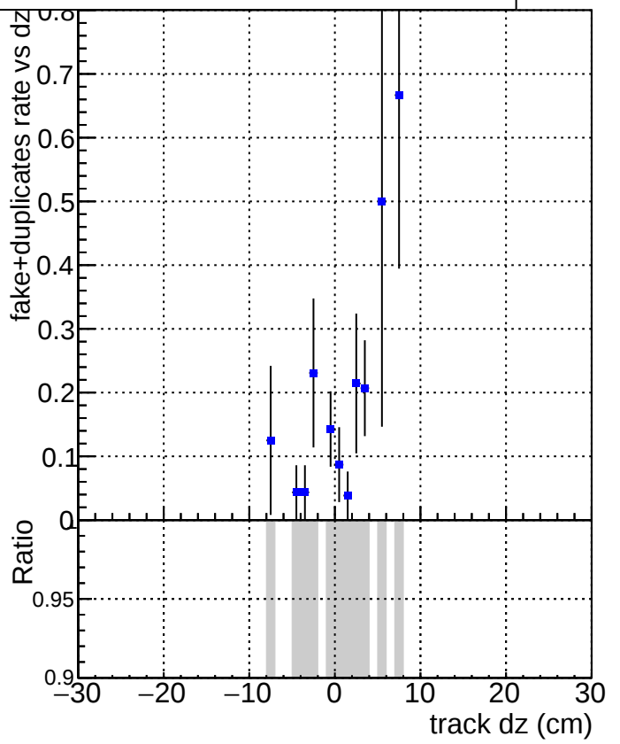
DQM_V0001_R000000001_Global_mkFiti100_RECO
