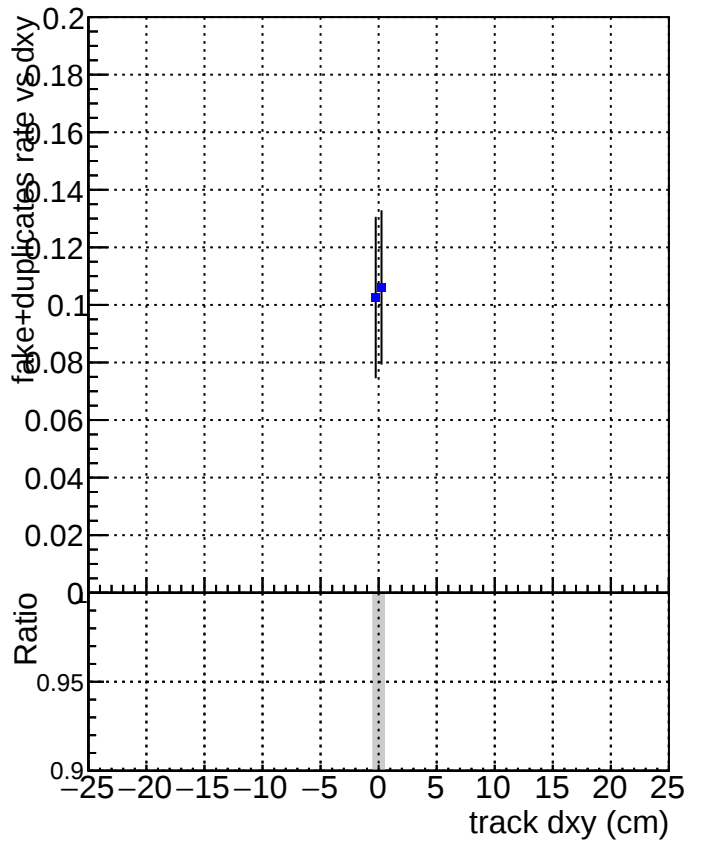
DQM_V0001_R000000001_Global_mkFiti100_RECO
