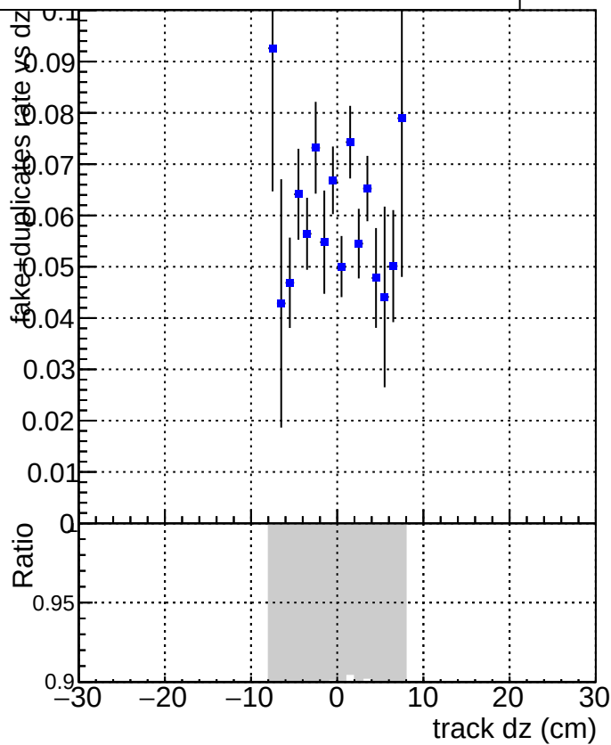
DQM_V0001_R000000001_Global_mkFiti100_RECO
