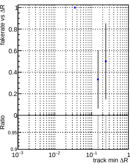
Fake rate vs \Delta R(\text{track, jet}) DQM_V0001_R000000001_Global_mkFiti100_RECO
