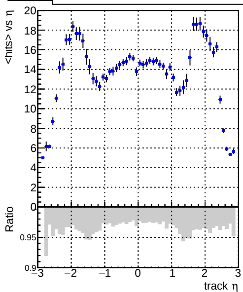
mean hit DQM_V0001_R000000001_Global_mkFit100_RECO
