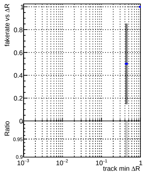
Fake rate vs \Delta R(\text{track}, \text{jet}) DQM_V0001_R000000001_Global_mkFiti100_RECO
