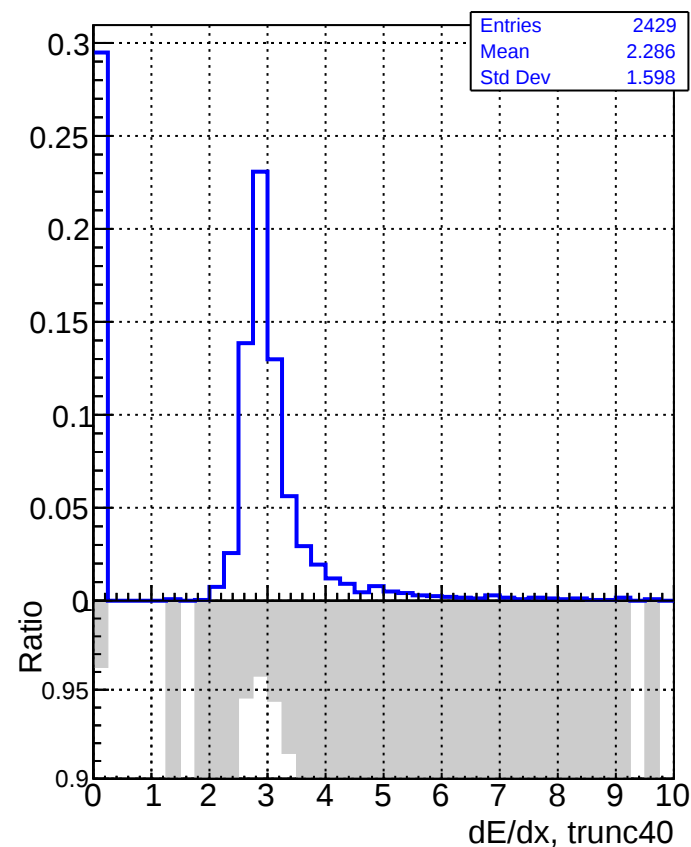
DQM_V0001_R000000001_Global_mkFiti100_RECO
