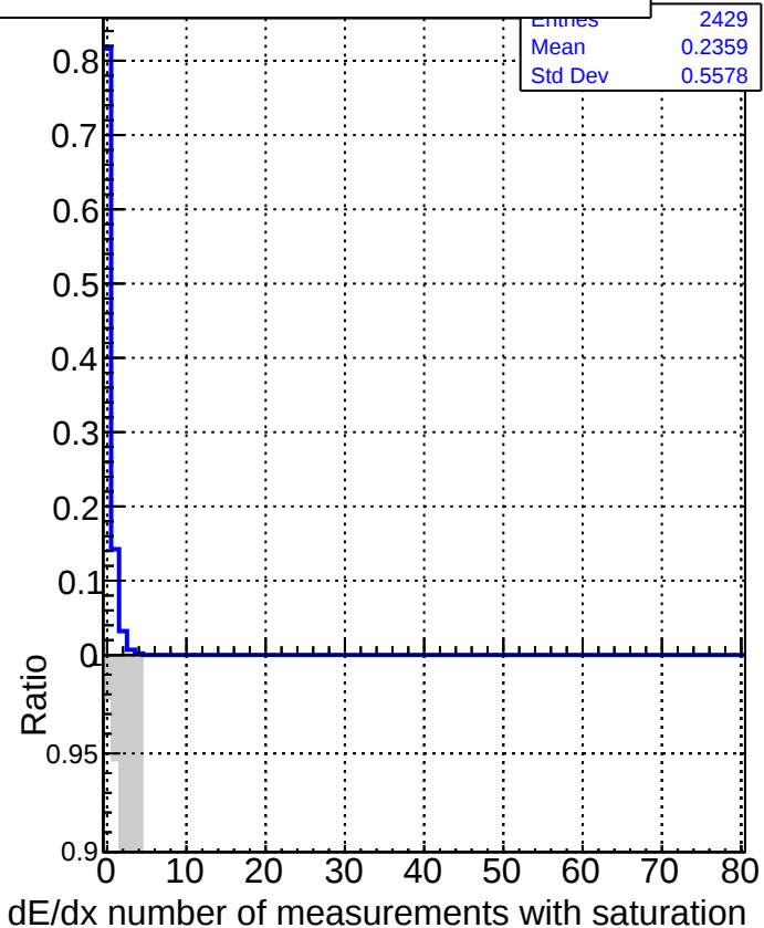
DQM_V0001_R000000001_Global_mkFiti100_RECO
