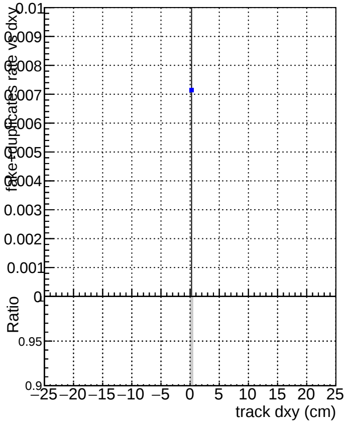
DQM_V0001_R000000001_Global_mkFitti100_RECO
