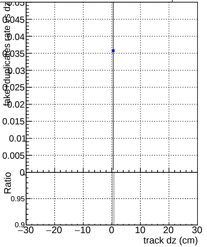
DQM_V0001_R000000001_Global_mkFitti100_RECO
