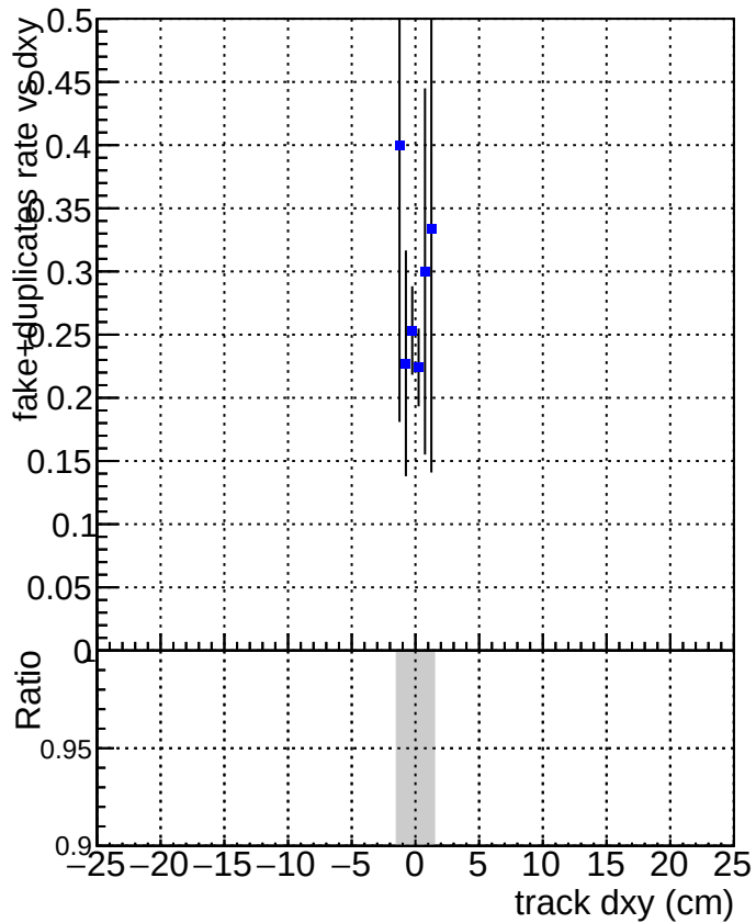
DQM_V0001_R000000001_Global_mkFiti100_RECO
