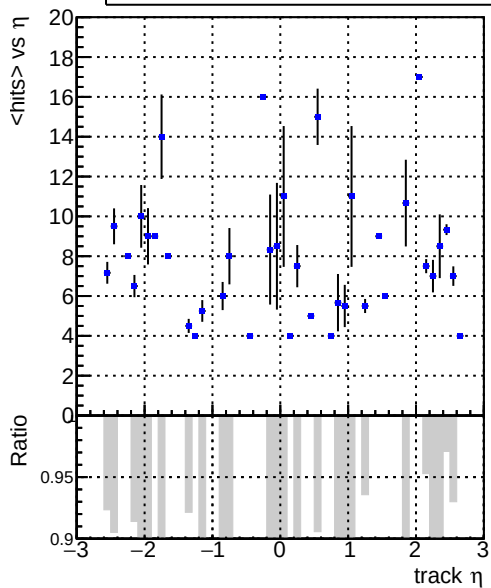
mean hits DQM_V0001_R000000001_Global_mkFit100_RECO
