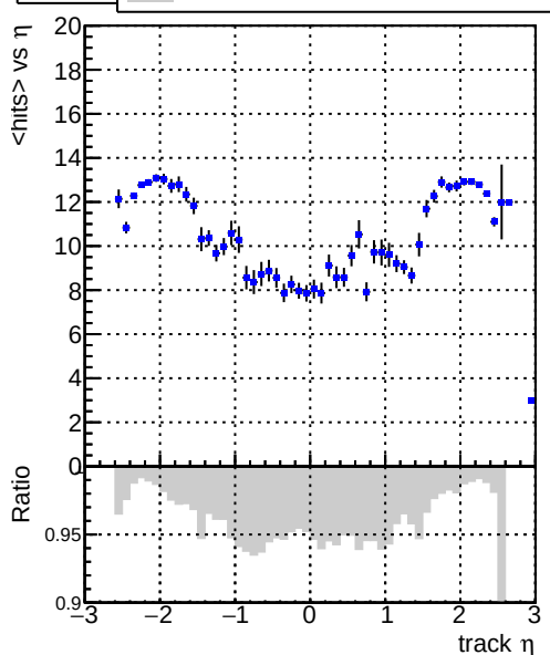
mean hits vs \eta DQM_V0001_R000000001_Global_mkFit100_RECO
