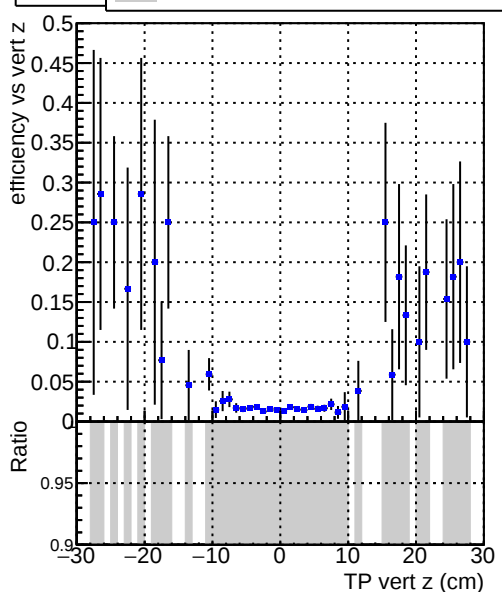
Efficiency vs. DQM_V0001_R000000001_Global_mkFit100_RECO
