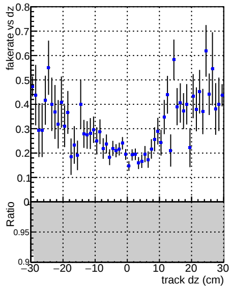
Fake rate vs dz —●— DQM_V0001_R000000001_Global_mkFit100_RECO
