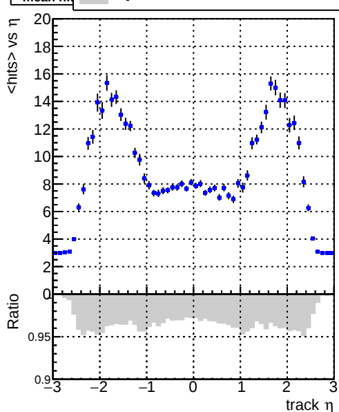
mean hits vs \eta DQM_V0001_R000000001_Global_mkFit100_RECO
