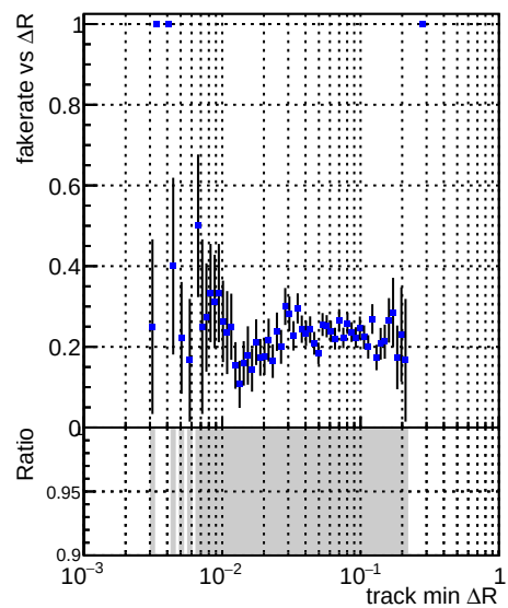
Fake rate vs \Delta R(\text{track, jet}) DQM_V0001_R000000001_Global_mkFiti100_RECO
