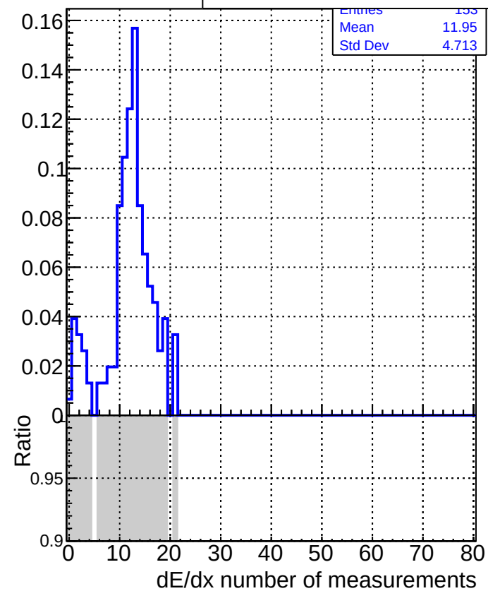
DQM_V0001_R000000001_Global_mkFiti100_RECO
