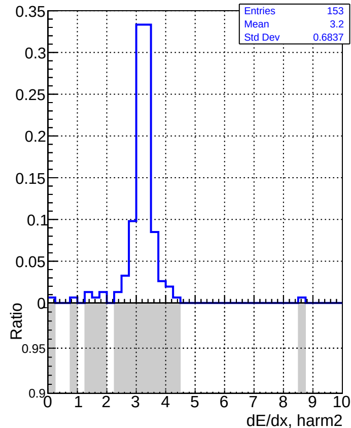
DQM_V0001_R000000001_Global_mkFiti100_RECO
