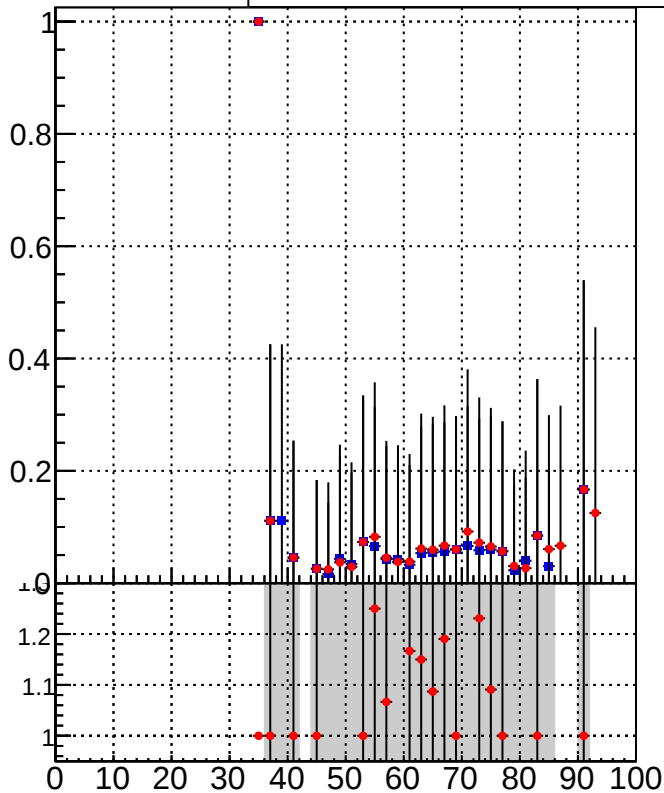
—■— DQM_TT_mkFit_ —●— DQM_TT_mkFit_BDT_
