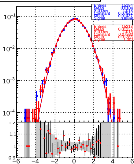
RecoAllAssoc2GenMatchedMerged_PulIX
