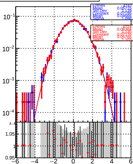
RecoPVAssoc2GenPVMatched_PulIX
