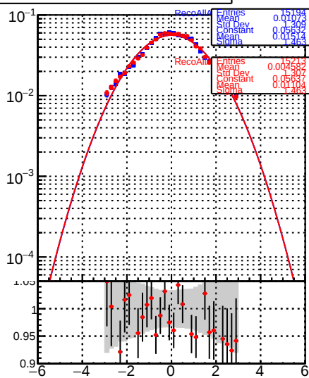
RecoAllAssoc2GenMatchedMerged_PulIZ
