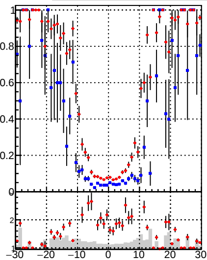
—•— DQM_TT_mkFit_ —•— DQM_TT_mkFit_BDT_
