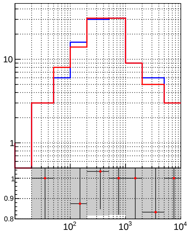
RecoAssoc2GenPVMatchedNotHighest_Pt2
